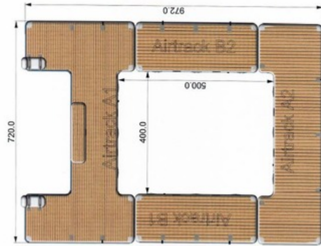
Drawing swimming dock with swimming pool - new in 2020
